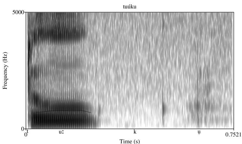
Figure 6: tuúku 'ear'
