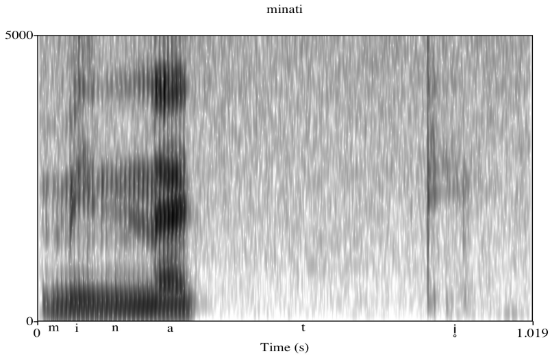
Figure 1: minati 'pineapple'
