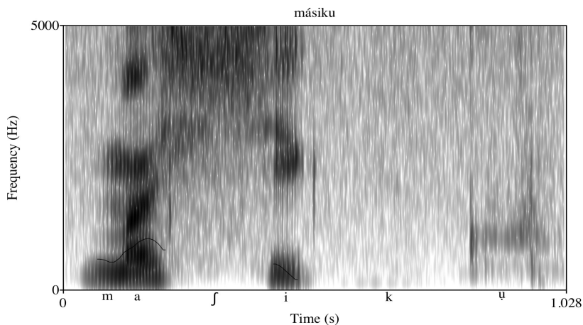
Figure 3: máʃiku 'raft'
