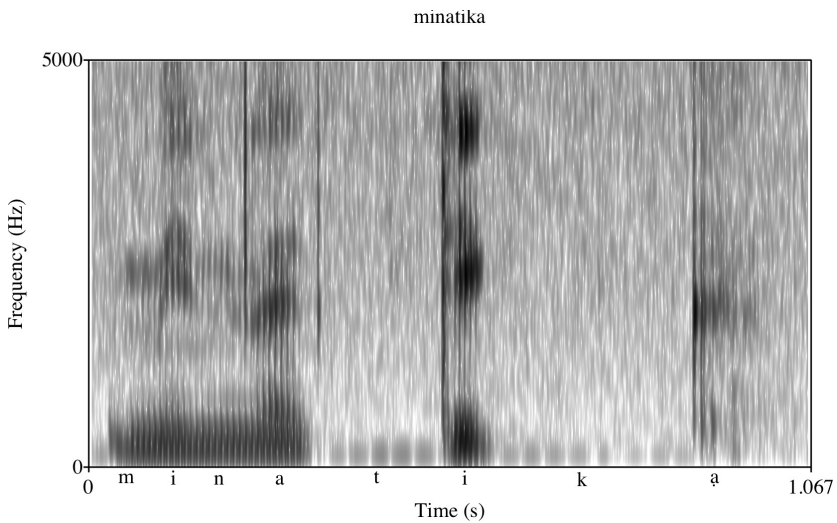
Figure 2: minatika 'pineapples'
