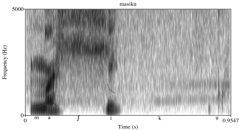
Figure 4: majiku 'paucar'
